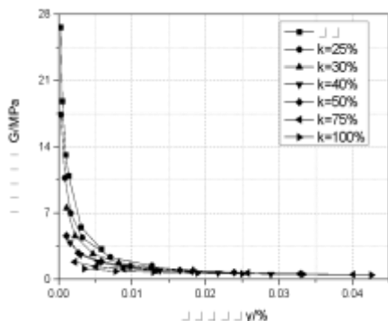
(a) Confining pressure 50kPa
