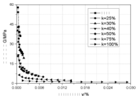
(c) Confining pressure 200kPa
