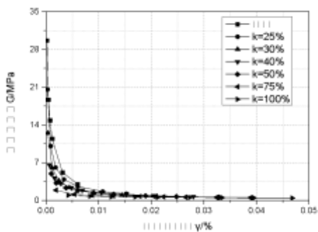
(a) Confining pressure 50kPa
