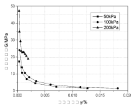
(b) Rubber particle content 25%
