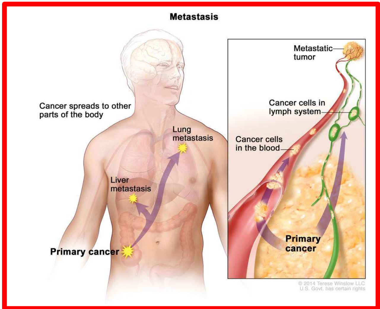
Figure 4: Cancer and metastasis by travelling through blood & lymph systems.
