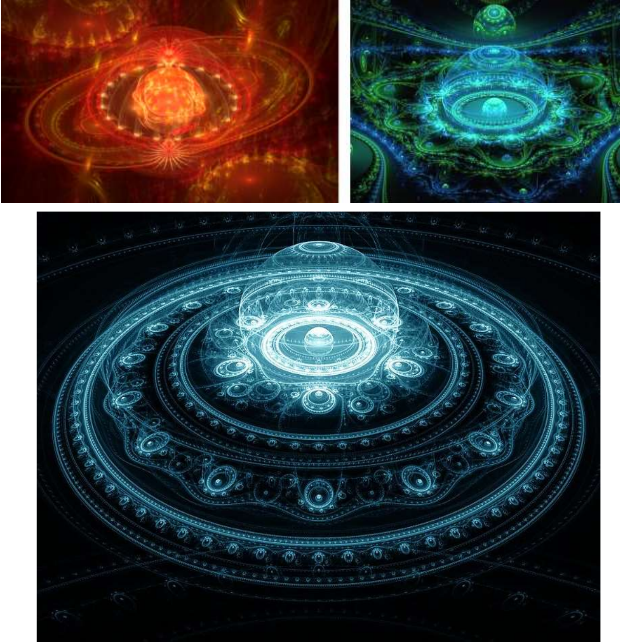
Fig. 8: Fractal illustrations of multi-layered raqiya (i.e., spherical abyss-crack), separating core of a "corpuscle" (in particular, "electron 10 ") from its outer shell
