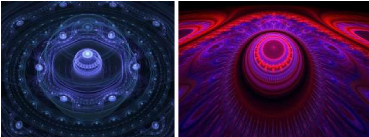
Fig. 10: Fractal illustrations of a raqiya (i.e., a spherical abyss-crack) surrounding the core of a "corpuscle," specifically, an "electron 10 "
