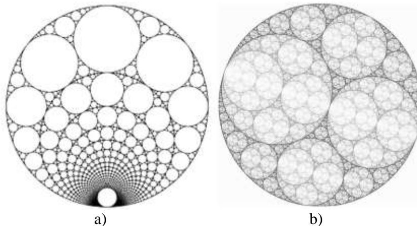
Fig. 4: Attempts to illustrate (using the "Apollo Circles" fractal) a multitude of hierarchical chains of cores nested within each other, starting with a single largest core (e.g., the core of a mega-Universe) and ending with a single smallest core (e.g., the core of an «instanton»).
