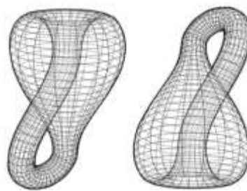
Fig. 5: Klein's bottle and anti-bottle
