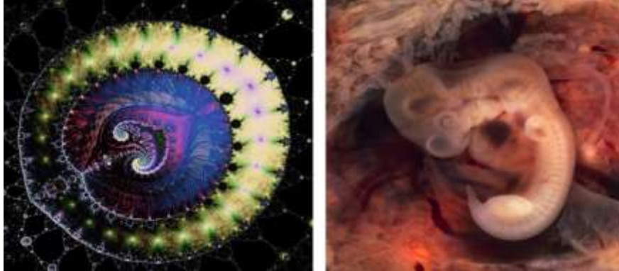
Fig. 17: Illustration of the development of the Embryo in the Universal Maternal Womb (i.e., in a Closed Cavity)
