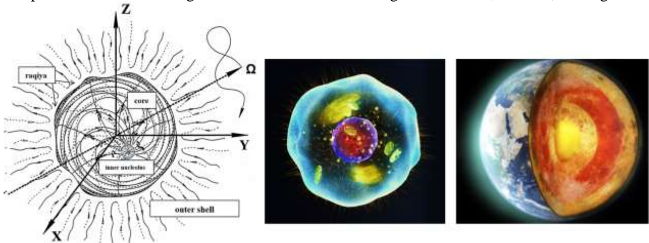
Fig. 16: Visual analogy between the bodily shells (core) of an "electron" (204) – (207), a biological cell, and a planet
