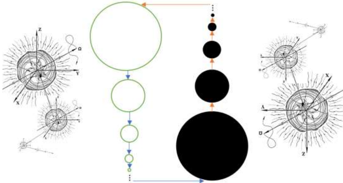
Fig. 2: Schematic representation of one of the closed hierarchical chains of “corpuscles” and “anticorpuscles” of various sizes (15), whose cores are nested inside one another like Russian nesting dolls
