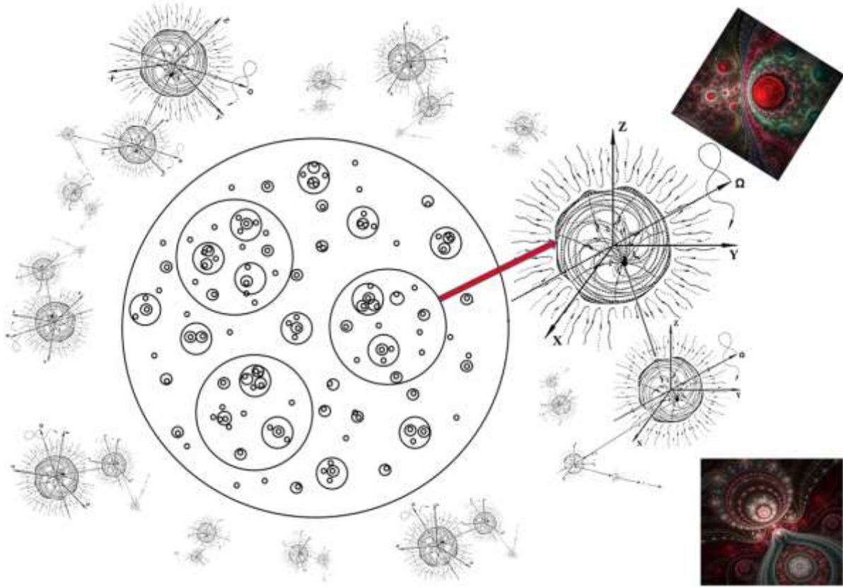
Fig. 1: A schematic representation of the “Hierarchical Cosmological Model,” consisting of an infinitenumber of hierarchical chains of “corpuscles” and “anticorpuscles” of various sizes, whose cores of different scales are nested within one another like Russian nesting dolls
