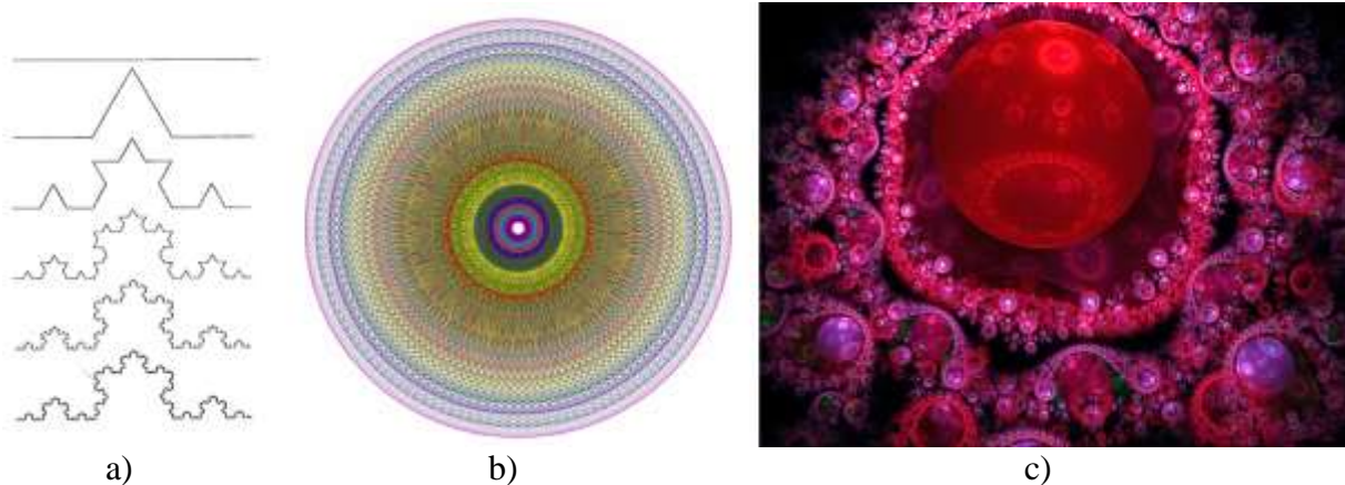
Fig. 9: a) The first six iterations of the "Koch curve" fractal; b) Increasing line irregularities as approaches the core (Prokhorov-Lebedev diagram); c) Fractal illustration of the increasingly complex vacuum curvature in the "corpuscles" raqiya as approaches its core, due to increasing finesse of the irregularities and decreasing radii of turbulent distortions.
