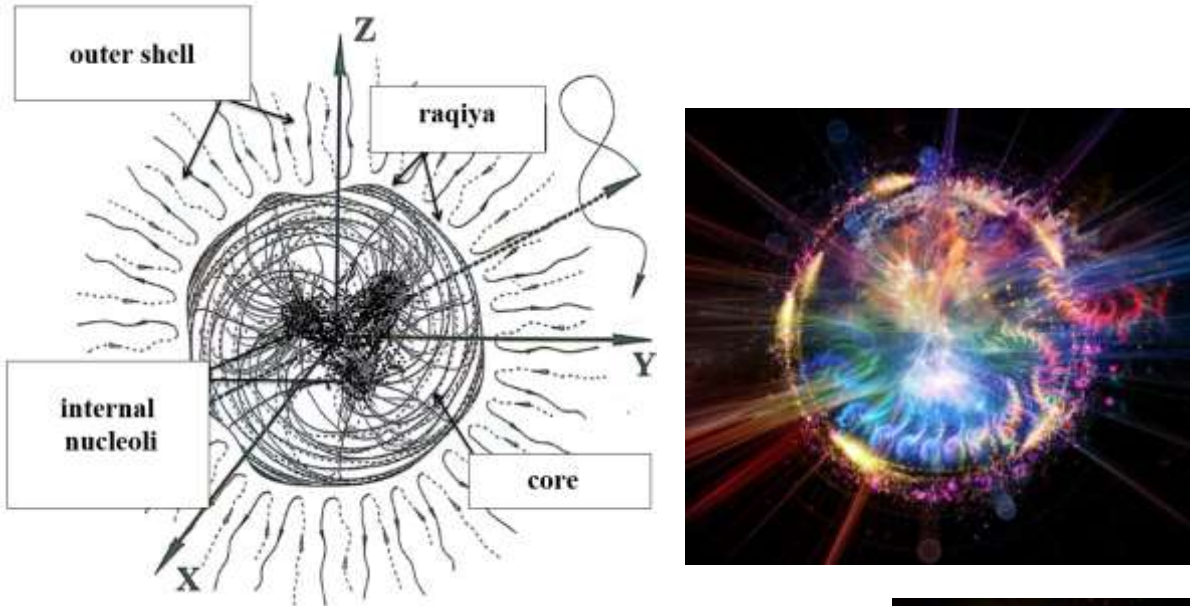
Fig. 11: Illustration of a concave on average spherical stable vacuum formation, consisting of two colored "antiquarks" and one "quark" (specifically, a p_i^- - "proton" (250)). The inner nuclei of these vacuum formations are in constant, chaotic motion relative to each other and relative to the common center of the p_i^- - "proton's" core
